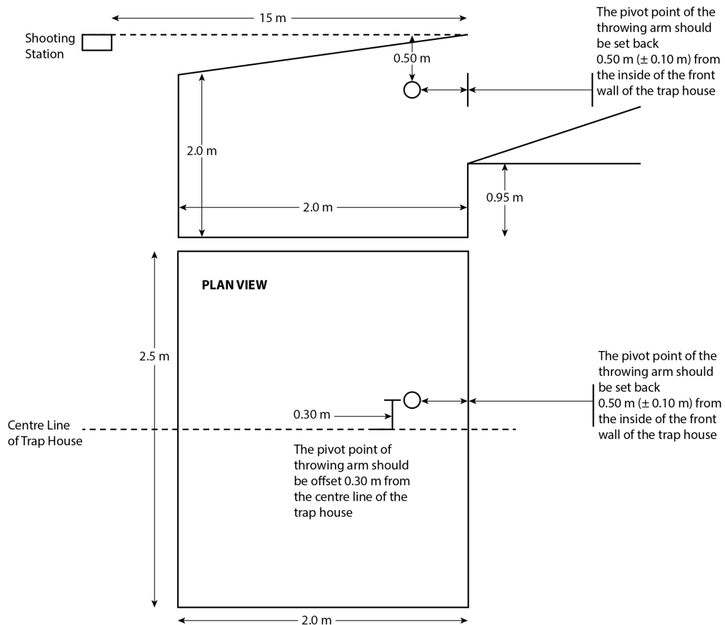
Ball Trap DRAWING NOT TO SCALE
