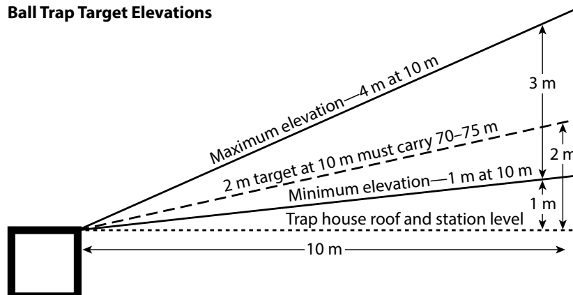
Ball Trap Target Elevations
