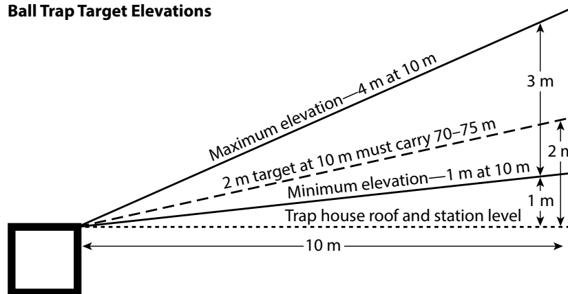
Ball Trap Target Elevations
