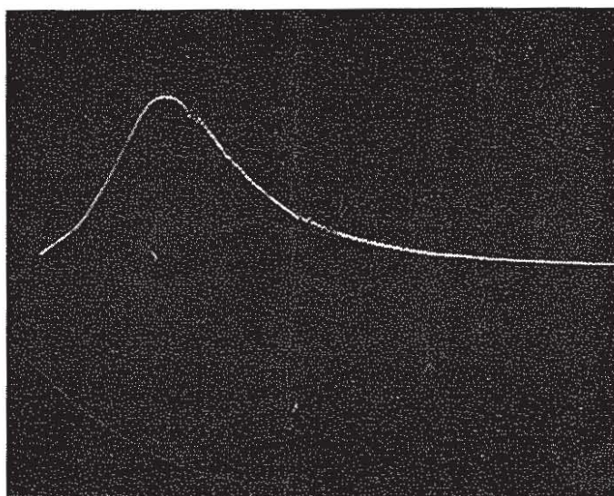
Fig. 2: A typical pressure-time curve for a shotgun cartridge.
