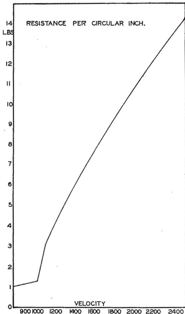
FIGURE 1 RESISTANCE OF THE AIR.
