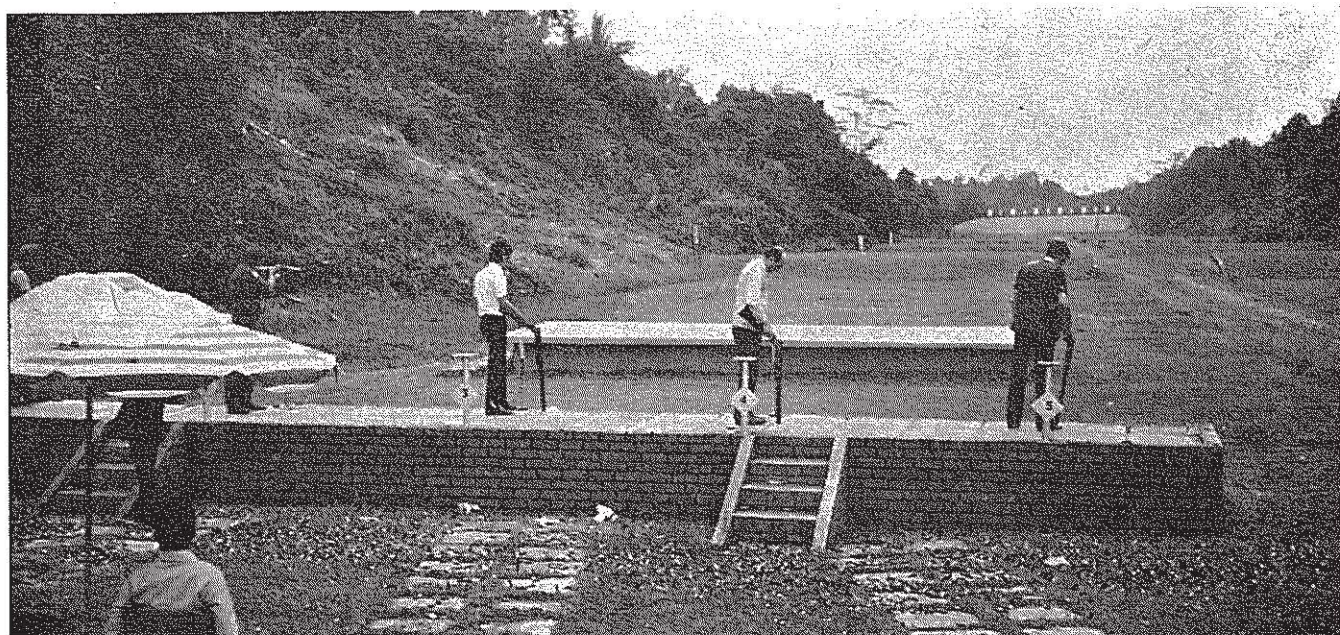
View down the trench range at Singapore showing the raised shooting pad in the foreground and the trench machine enclosure in the background.
