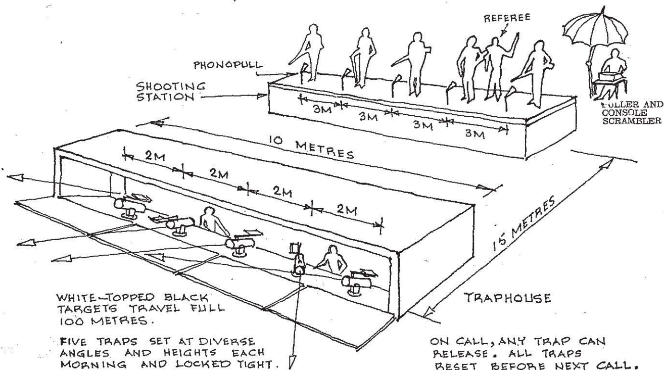
Singapore trench layout.
