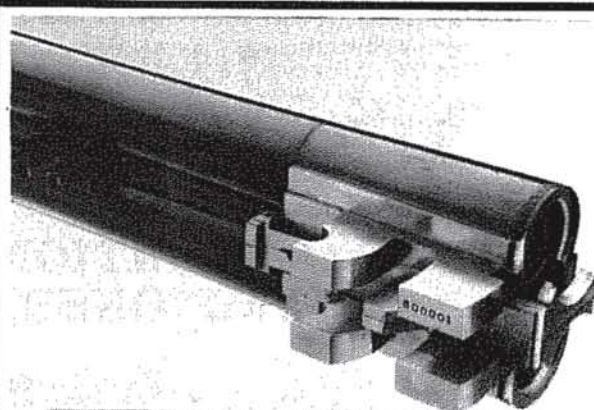
"Detail of double-lug mono-lug system"
