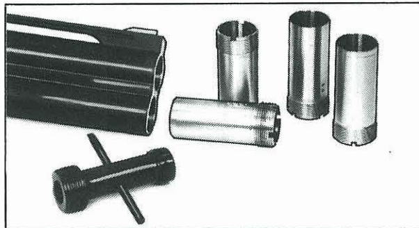
New flush mounting choke system that does not alter line of barrels. 4 chokes imp. cyl., mod., imp. mod., — and full. Key/thread cleaner come with guns featuring the mobilchoke system.
