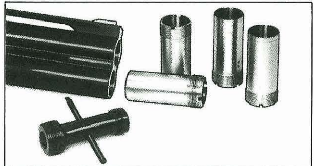
New flush mounting choke system that does not alter line of barrels. 4 chokes imp. cyl., mod., imp. mod., — and full. Key/thread cleaner come with guns featuring the mobilchoke system.
