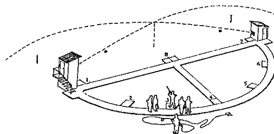
Skeet Ground Layout
