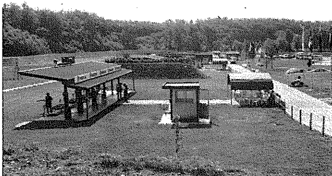
Shooting grounds, Fagnano, Italy - 6 layouts.
