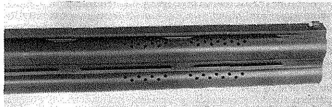
The porting patterns on the barrels of the Super Trap have been reported to reduce recoil significantly and tame muzzle flip by up to 40%.
