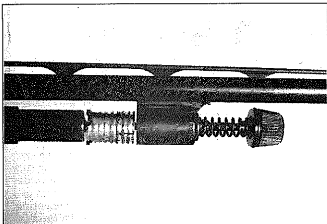
With the forend removed, the gas system is quite basic in design but very effective in reducing recoil
