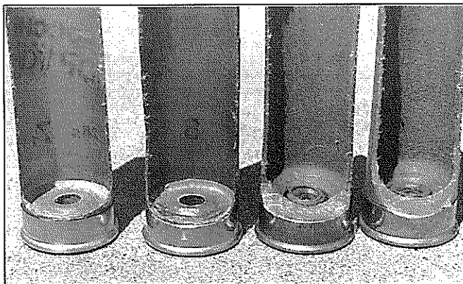
Sectioned cases. The two on the left are Reiffenhauser; on the right are compression moulded Winchesters. It's fairly obvious that the Reiffenhauser type has greater capacity.
