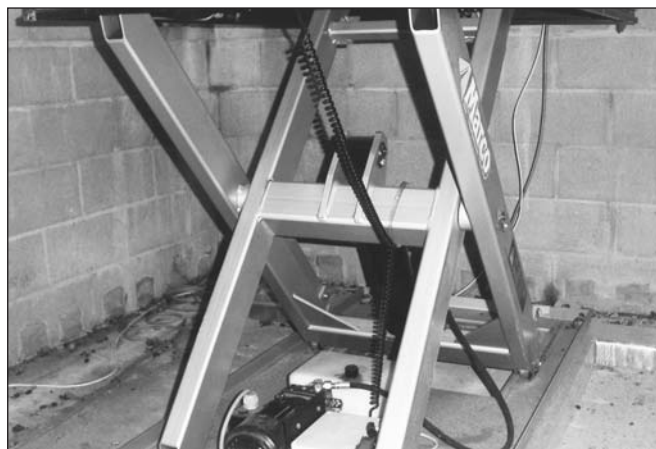
The hydraulically operated scissor lift raises and lowers the Trap House to any selected level. Roller guides stabilise the platform against the walls of the pit.
